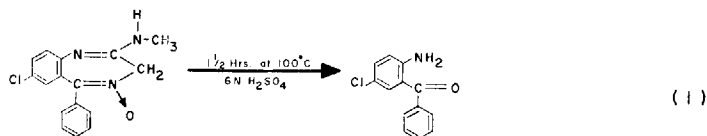
CHLORDIAZEPOXIDE
