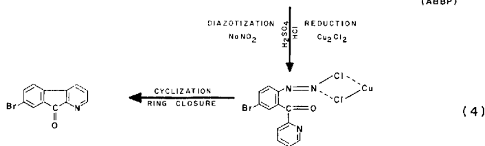
"FLUORENONE" DERIVATIVE
